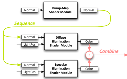
Fig. 2. The output values of three simple shaders can be combined with two composition operators: Sequence and Combine(operator +) .
