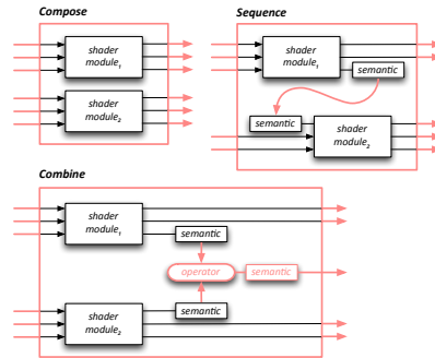
Fig. 3. The three semantic-aware basic composition operators for shader composition. For illustration purposes, the Sequence function is depicted with only one semantic routed between its shader module arguments.
